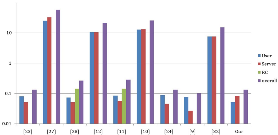
Fig. 7 Execution time (in logarithmic scale)
