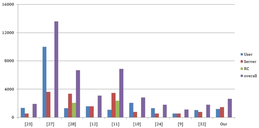
Fig. 8 Communication cost (in normal scale)
