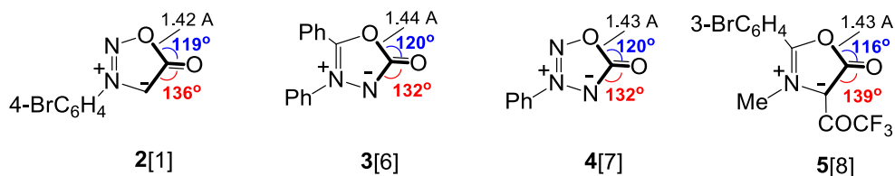
Fig. 1 X-ray determined geometries of type A mesoionic rings with an exocyclic C=O group
