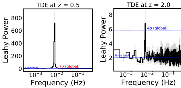
Fig. 11 Simulated power density spectra of an ASASSN-14li-like TDE at various redshifts using Athena's Wide Field Imager (WFI). For each of these simulations we used an exposure time of 32 ks and a QPO fractional rms amplitude of 40% (similar to ASASSN-14li) whose value remains constant with energy within 0.3–2 keV bandpass. Statistical confidence contours and the Poisson noise level of 2 are shown as dashed horizontal lines. The time dilation effect due to the redshift and the potential well of the source on the centroid frequency of the QPO was neglected as it will not alter the results significantly. Assuming ASASSN-14li-like behavior, TDE X-ray QPOs could be detected out to a redshift of roughly 2 with a meter-class X-ray telescope
