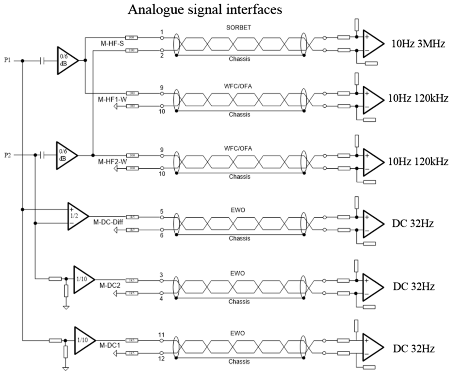
Fig. 10 MEFISTO analogue interfaces
