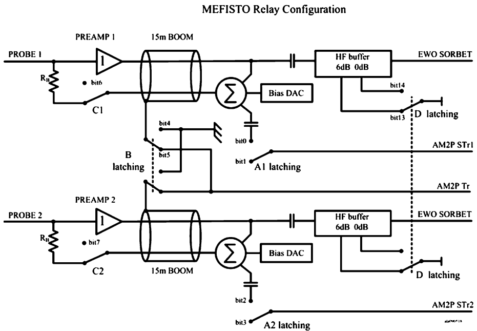
Fig. 9 Illustration of the simplified MEFISTO signal paths and controls
