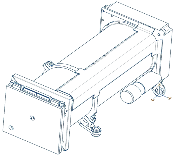
Fig. 6 MEFISTO boom unit, outside view (Blomberg et al. 2006)
