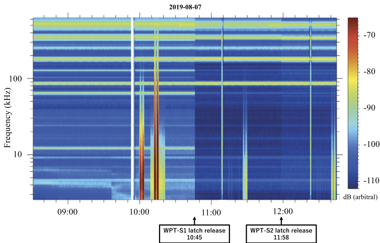
Fig. 13 Noise floor changes seen in PWI SORBET spectrum during the WPT-S latch release operations on 7 August 2019. The latch release action of WPT-S1 and WPT-S2 were at 10:45 UT and 11:58 UT, respectively
