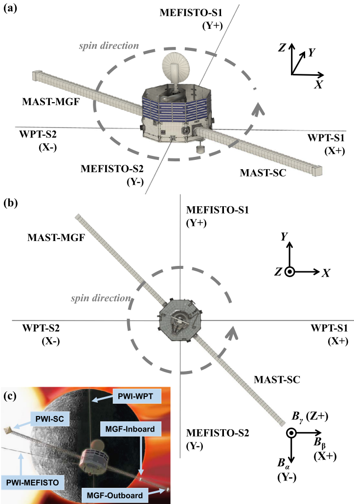
Fig. 3 Location of MEFISTO and WPT sensors on the Mio spacecraft. (a) External view, (b) view along the spin axis (+Z), and (c) a schematic view. The spacecraft coordinates and the direction of the spacecraft spin rotation (spin rate: 4–5 sec) are also shown. (From Kasaba et al. 2020)
