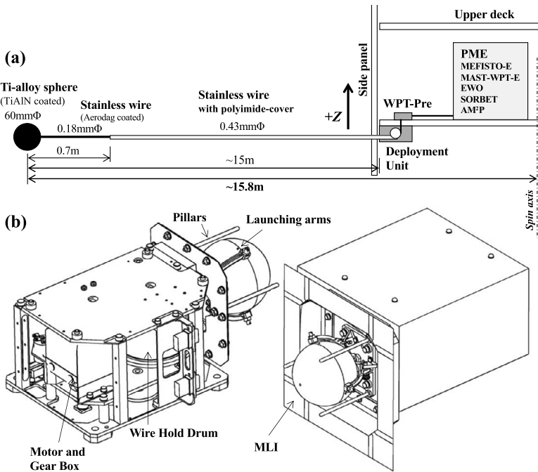
Fig. 11 Design of WPT-S. (a) Geometry. (b) Schematic drawing. To the left the mechanics of the deployment unit is shown. To the right is the outer view covered by MLI. (b) is courtesy of Nippi Corporation
