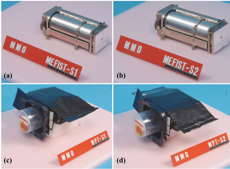
Fig. 1 Pictures of PWI wire antenna booms at the shipment to the system in 2012. (a) MEFISTO-S1, (b) MEFISTO-S2, (c) WPT-S1, (d) WPT-S2
