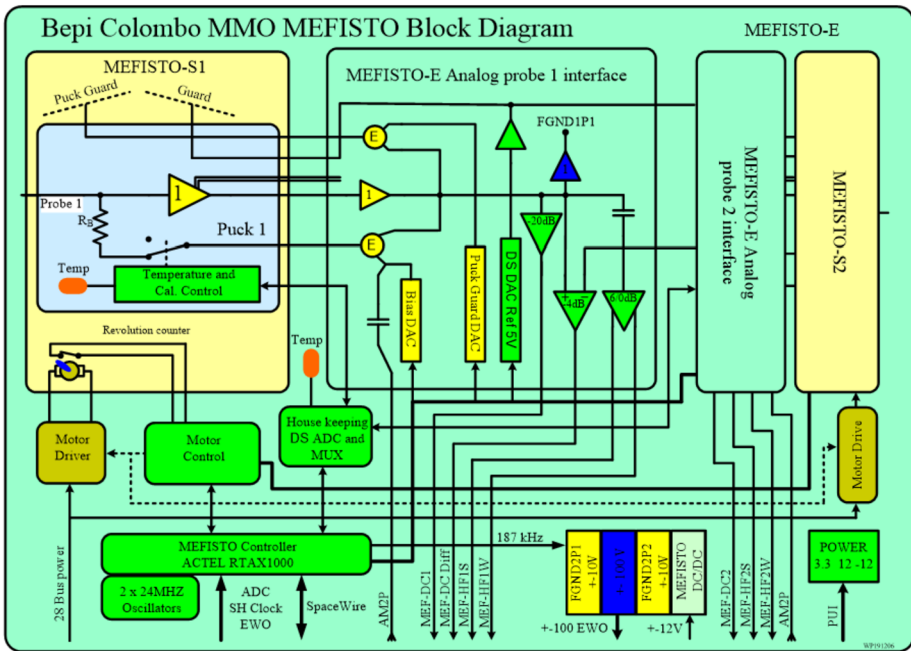
Fig. 7 MEFISTO block diagram
