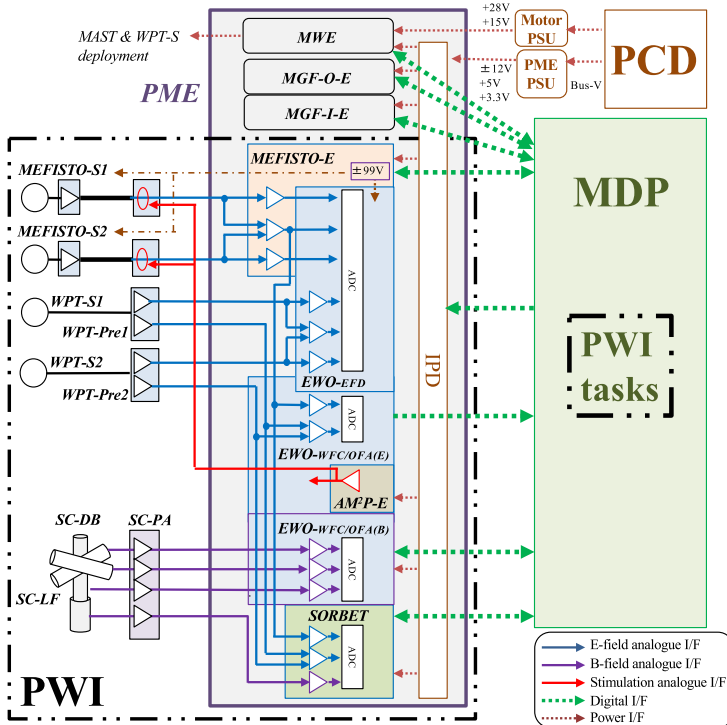
Fig. 2 MEFISTO and WPT in the PWI system. Characteristics of the I/F lines are summarized in the drawing. The deployment of MEFISTO and WPT are controlled by MEFISTO-E and MAST-WPT-E in the PME chassis. (From Kasaba et al. 2020)
