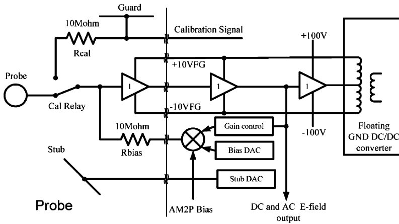
Fig. 8 MEFISTO floating ground concept
