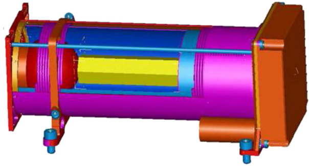
Fig. 5 MEFISTO boom unit, interior view (Blomberg et al. 2006)
