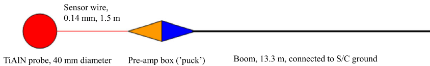
Fig. 4 MEFISTO sensor configuration. Adapted from Blomberg et al. (2006)
