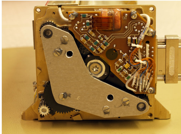
Fig. 12 Photo of the AM 2 P-S current probe, hosted in the MEFISTO deployment box, designed to measure the current in the MEFISTO wire boom shield
