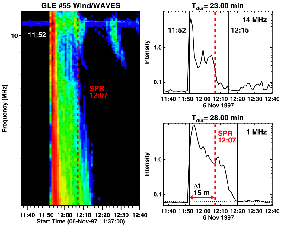
Fig. 8 WAVES dynamic spectrum ( left ) and the frequency cuts at 14 MHz ( top right ) and 1 MHz ( bottom right ) for the type III burst associated with the 1997 November 6 GLE. The intensity is in units of microvolts per \sqrt{\text{Hz}} . Horizontal dotted lines show the 5-sigma limit, which needs to be exceeded for the burst onset. The vertical solid lines mark the duration of the type III burst. The SPR time (12:07 UT) and the delay time ( \Delta t = 15 min) of SPR with respect to the type III onset are marked on the plots. Note that the SPR happens towards the end of the type III interval
