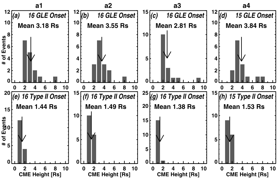
Fig. 14 CME heights at SPR (upper panels, a–d) and at metric type II burst onset (lower panels, e–h) obtained using the four different accelerations a_1 – a_4 . CME heights were assuming that the CME accelerates from the flare onset time (see Fig. 10) with an initial height of 1.25 R_s
