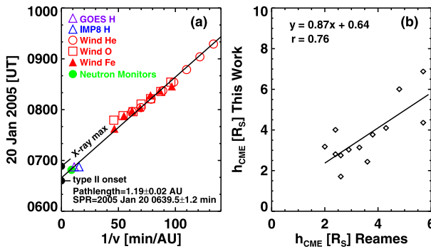
Fig. 17 (a) Velocity dispersion plot for the 2005 January 20 event from Reames (2009a). (b) Scatter plot between the CME heights ( h_{CME} ) obtained by the velocity dispersion method (Reames 2009a) and by assuming the path length as 1.2 AU (this work) showing good correlation (correlation coefficient r = 0.76 ). Our h_{CME} = h_{4G} in Table 2 except for the six cases where linear extrapolation was possible (values in parentheses in the h_{4G} column of Table 2)
