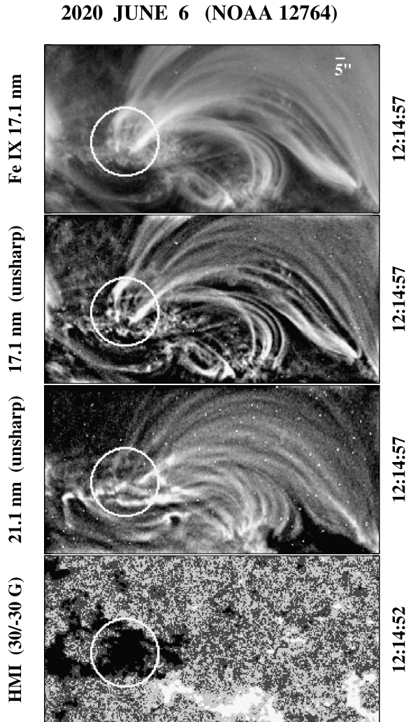
Figure 3 AR loop system (NOAA 12764) observed on 2020 June 6, at the onset of Solar Cycle 25. Within the circled area (of radius 18'' ), looplike features with dimensions on the order of 5'' may be seen at the footpoints of the longer loops. These features are embedded in the 17.1-nm moss overlying the negative-polarity plage.
