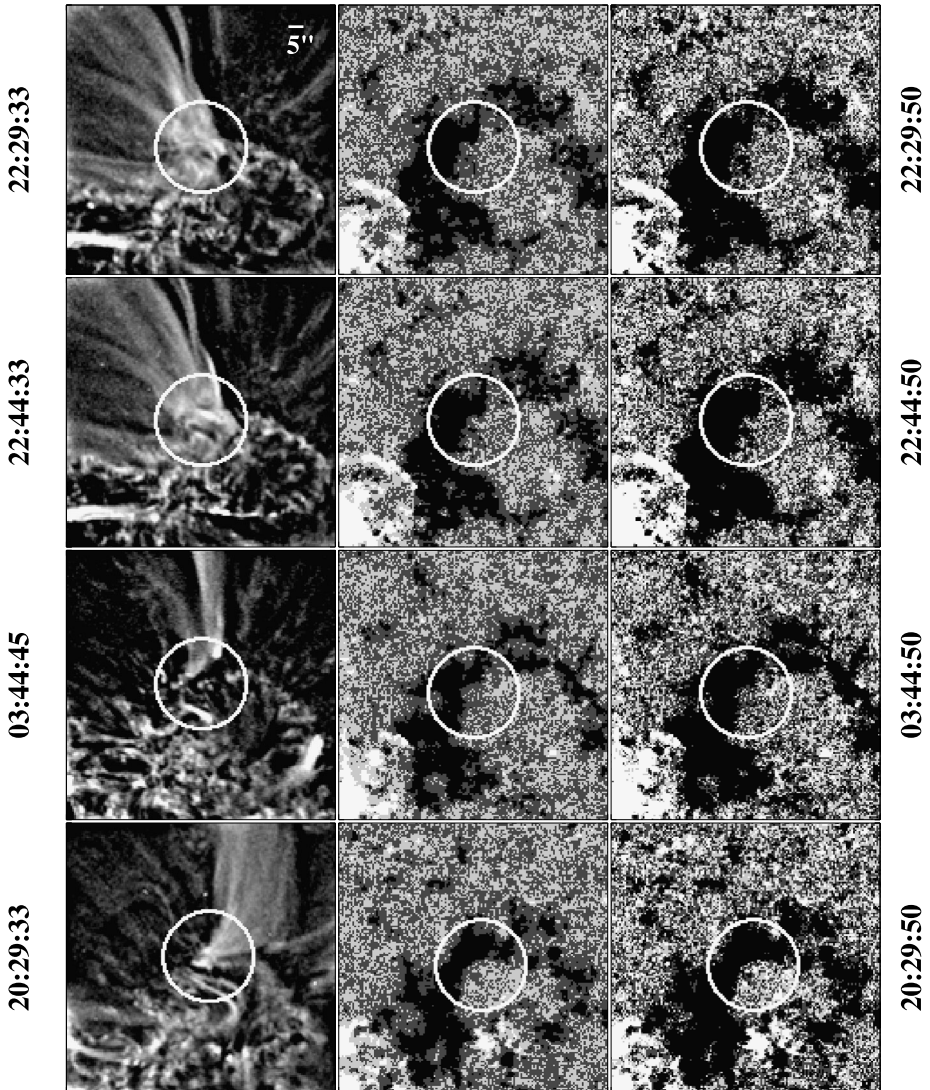
Figure 4 Evolution of 17.1-nm loops inside NOAA 12823, 2021 May 13–14. As the underlying plage area narrows, the cluster of AR loops present late on May 13 fades and is replaced by a smaller bundle on May 14. Relatively large ( \gtrsim 5'' ) looplike features may be seen at the base of the AR loops; some of these footpoint structures have at least one leg located above the weak, mixed-polarity region on the west side of the negative-polarity plage. The magnetograms in the rightmost column have been saturated at \pm 10 G instead of \pm 30 G (as in the middle column ), so that light and dark gray pixels here indicate locations where B_{\text{los}} is close to the HMI noise level.
