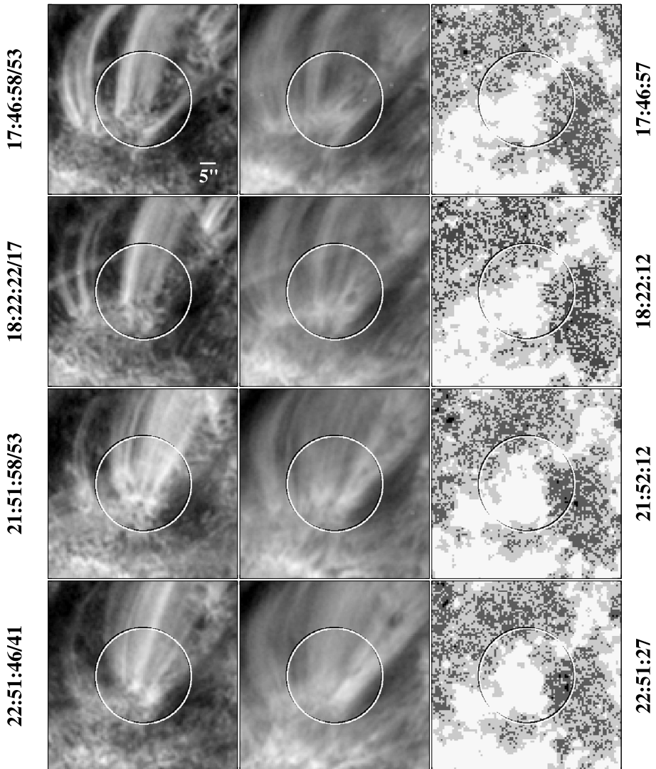
Figure 1 A cluster of coronal loops observed inside NOAA 12443 late on 2015 November 5. The circled area has a radius of 15'' . The Fe IX 17.1-nm ( left column ) and Fe XII 19.3-nm ( middle column ) loops are rooted in moss overlying a plage area containing only positive-polarity flux, according to the corresponding HMI magnetograms ( right column ). The brightness and spatial distribution of the 17.1-nm loops vary continually over the 5-hour period, as does the underlying fine structure, which, in addition to dark chromospheric material, consists of looplike features and compact brightenings that appear to be an integral part of the moss. The emission is more diffuse and widespread in the 19.3-nm images (recorded 5 s before the 17.1-nm images). Movies suggest that the fading of the Fe IX loops is often accompanied by downflows (see the animation accompanying Figure 10 in Wang, Ugarte-Urra, and Reep, 2019). Here, and in subsequent figures, the gray scale used in the magnetograms is as follows: white ( B_{\text{los}} > 30 G), light gray ( 0 \text{ G} < B_{\text{los}} < 30 G), dark gray ( -30 \text{ G} < B_{\text{los}} < 0 G), black ( B_{\text{los}} < -30 G).
