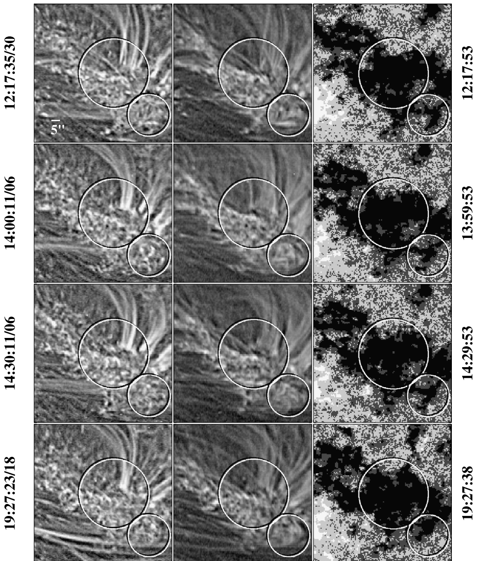
Figure 2 Small loop-shaped features embedded within the moss/plage inside NOAA 12351, as observed on 2015 May 23. Left column: Fe IX 17.1-nm images recorded at 12:17:35, 14:00:11, 14:30:11, and 19:27:23 UTC. Middle column: Fe XII 19.3-nm images recorded at 12:17:30, 14:00:06, 14:30:06, and 19:27:18 UTC. Right column: line-of-sight HMI magnetograms recorded at 12:17:53, 13:59:53, 14:29:53, and 19:27:38 UTC and saturated at \pm 30 G. An unsharp mask has been applied to the EUV images. Note that the moss-like structure and looplike features extend into the mixed-polarity, weaker-field areas beyond the plage itself, as indicated for example by the circled region at the southwest corner of the images. Loop-shaped structures with dimensions of a few arcseconds may be discerned not only in Fe IX but also in Fe XII, as near the center of the large circles in the 19.3-nm images taken at 14:00 and 14:30 UTC.
