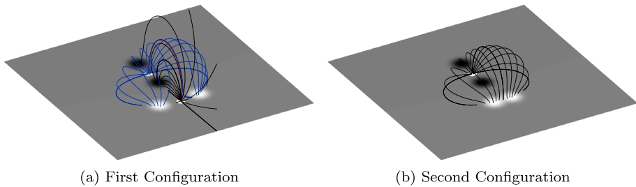
Figure 6 A four-source topology with circular sources of magnetic flux. (a) None of the sources overlap and each pair has a null point between them. (b) The positive sources now overlap. When compared to Figure 5b, it is clear that the null point is lost in the overlap.
