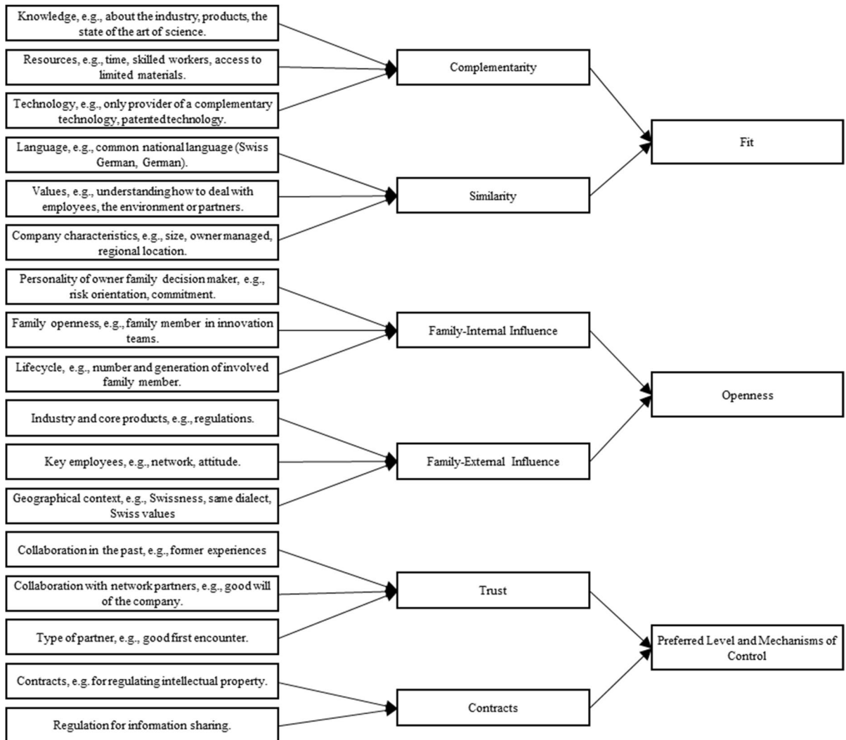
Fig. 1 Data structure
