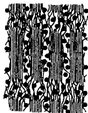
Swollen cellulose matrix with incorporated solvent molecules
