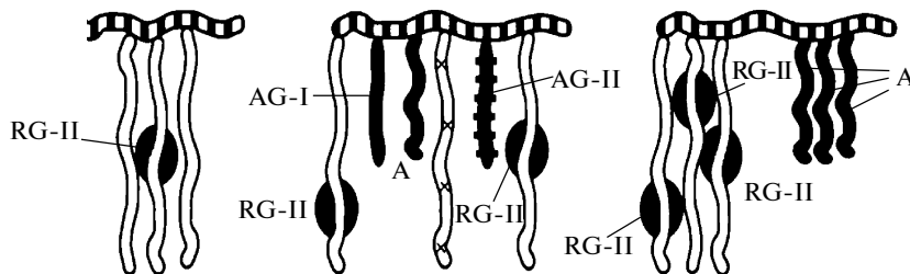
Schematic representation of a family of pectic polysaccharides
