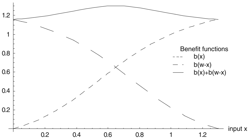
Fig. 4 The two expected benefit functions together with the objective function for a high value of w
