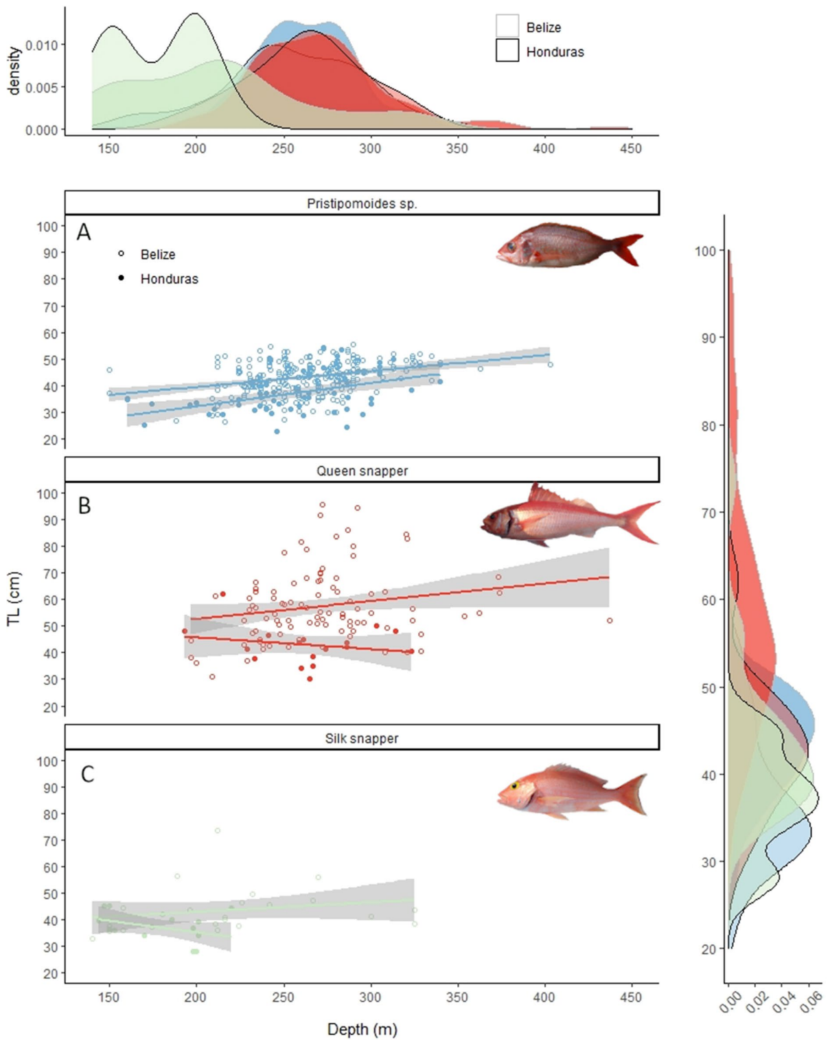
Fig. 7 Length-at-capture depth for A Pristipomoides sp.; B queen; and C silk snappers captured by fishery-independent methods with lines representing trends of GLMs by country
