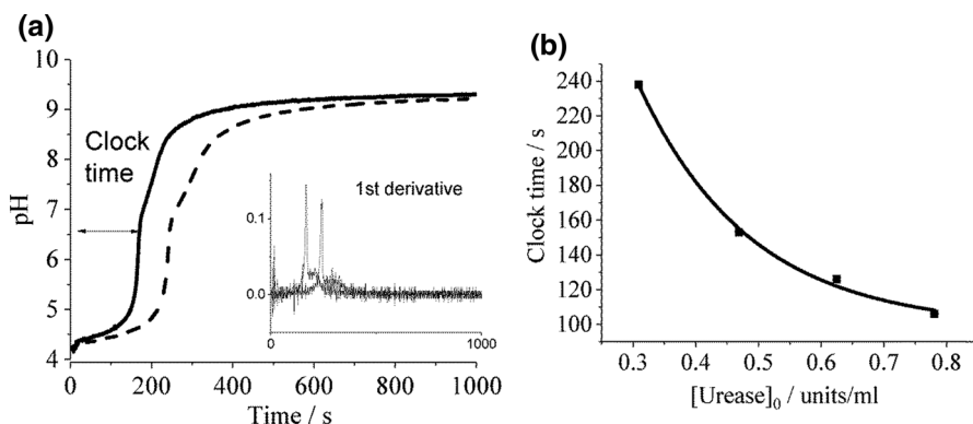
Fig. 1 a pH-time curves obtained for urea–urease reaction in a batch reactor for following conditions: [\text{urea}]_0 = 3.09 mM, [\text{HCl}]_0 = 0.125 mM, [\text{urease}]_0 = 0.469 units/ml (solid), [\text{urease}]_0 = 0.309 units/ml (dash). Inset shows first derivative used to calculate clock time and b a plot of clock time vs initial concentration of urease (curve shows exponential fit to data y = Ae^{-kx} + B with A = 786 , k = 5.6 and B = 98 )
