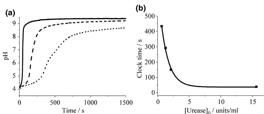
Fig. 4 a pH curves obtained for urea–urease reaction in batch reactor with different amounts of polymer beads added for initial conditions: [\text{urea}]_0 = 3.09 mM and [\text{HCl}]_0 = 0.125 mM, and the calculated activity of urease was: [\text{urease}]_0 = 15.6 U/ml (solid), [\text{urease}]_0 = 2.11 U/ml (dash), [\text{urease}]_0 = 0.632 units/ml (dot). b A plot of clock time vs calculated activity of enzyme (curve shows fitted exponential decay: y = Ae^{-kx} + B with A = 662 , k = 0.79 and B = 37 )
