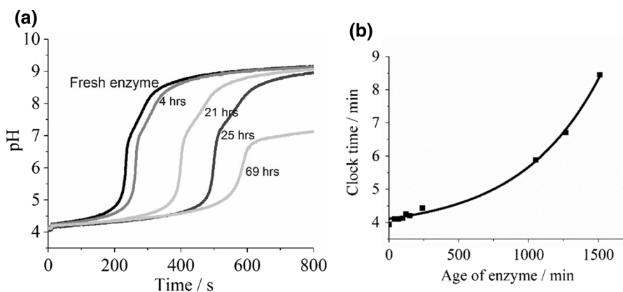
Fig. 2 a pH curves obtained for different ages of enzyme stock solution and b a plot of age of enzyme stock solution versus clock time (curve shows exponential fit to data y = Ae^{kx} + B with A = 0.33 , k = 0.0175 and B = 3.8 ). Initial conditions were: [\text{urea}]_0 = 3.09 mM, [\text{HCl}]_0 = 0.125 mM and [\text{urease}]_0 = 0.309 U/ml (at age = 0 h)
