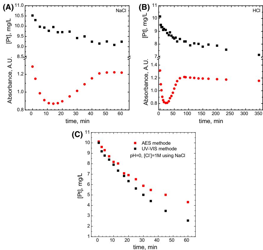
Fig. 9 Kinetic curves registered using AES and UV–VIS methodes, a chloride ion concentration controlled by addition 0.1 M NaCl, b chloride ion concentration controlled by additon 0.1 M HCl, C chloride ion concentration controlled by addition 1 M NaCl. Experimental conditions: [Pt(IV)] = 5 \times 10^{-5} M, [AC] = 1.67 g/L, T = 323 K, Mr = 1200 rpm
