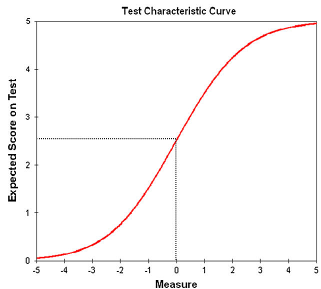
Fig. 1 Expected score
