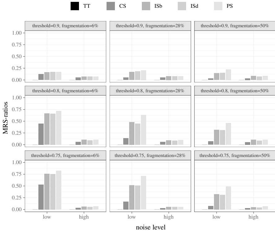
Fig. 4 MRS-ratios for the fuzzy-set experiment
