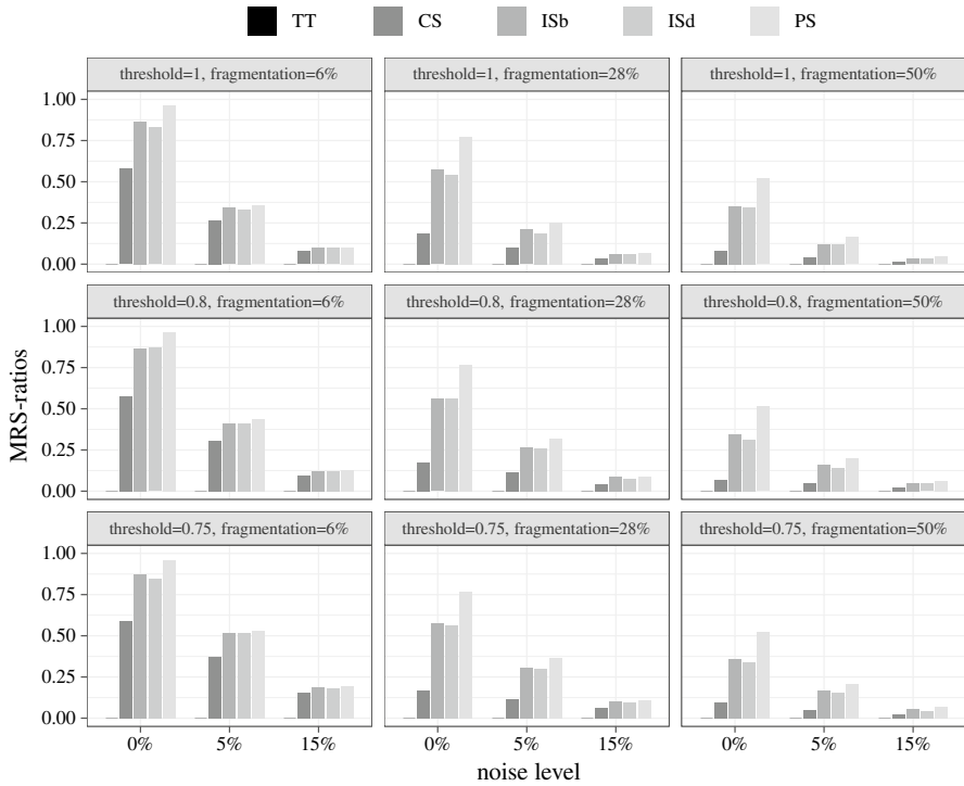
Fig. 2 MRS-ratios for the crisp-set experiment
