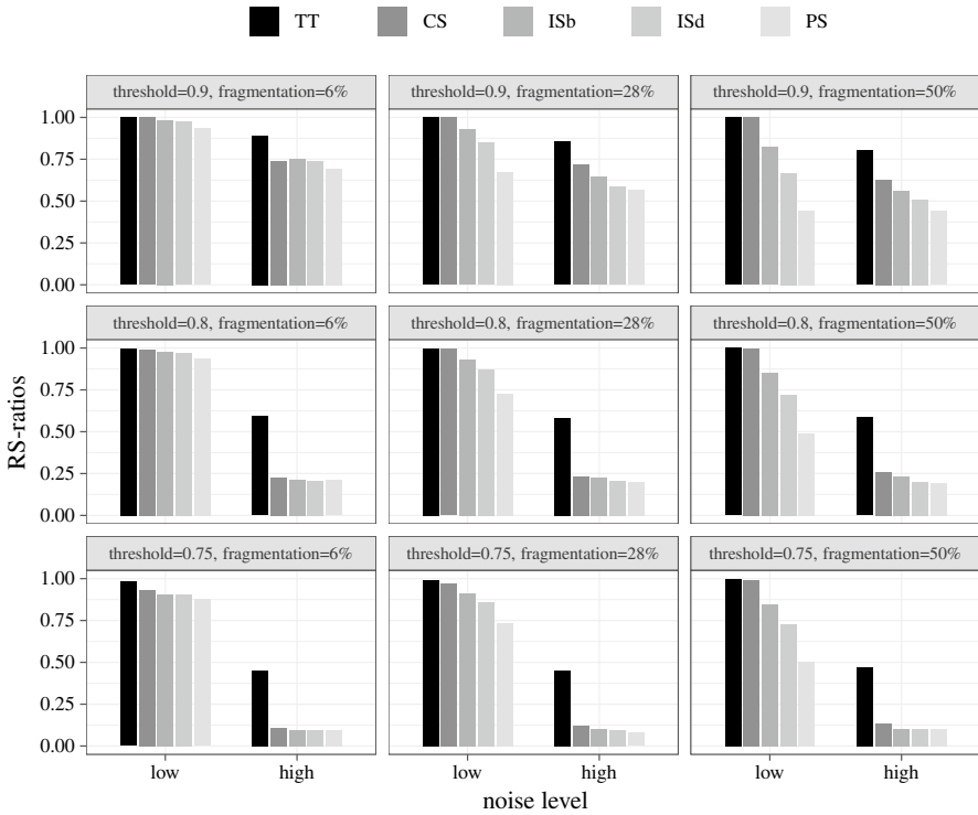
Fig. 3 RS-ratios for the fuzzy-set experiment
