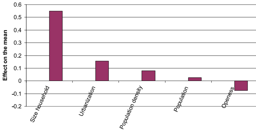
Fig. 7 Effect on the mean of the exploratory variables
