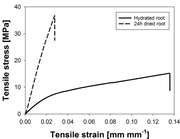
Fig. 1 Typical tensile stress versus tensile strain curves for a hydrated root sample ( d = 1.48 mm; w = 1.89 \text{g g}^{-1} ) and a root sample air-dried for 24 h ( d = 1 mm (before drying 1.40 mm); w = 0.11 \text{g g}^{-1} )
