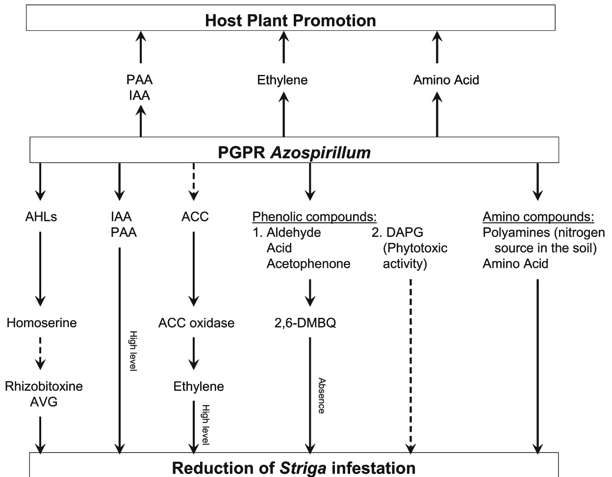
Fig. 3 Hypothetic molecular impact of PGPR Azospirillum in the tripartite interaction Azospirillum /Host plant/ Striga spp. 1-amino-cyclopropane-1-carboxylate (ACC), Acyl-homoserine lactone (AHLs), Aminoethoxyvinyl Glycine (AVG), Diacetylphlorogluci-
