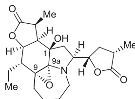
82 tuberostemonoxirine Yue et al. 2013
