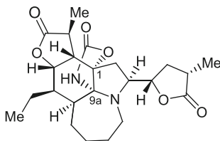
83 stemoxazolidinone E Hitotsuyanagi et al. 2011
