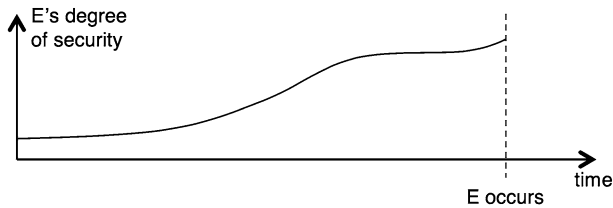
Fig. 1 The graph illustrated here shows a typical evolution of an event's security over time: at times long before E 's occurrence, E has a very low degree of security, i.e. if things had been just slightly different at these times, E would not have occurred. Closer to E 's occurrence, however, E 's degree of security begins to grow, and just before E 's occurrence, E has a quite high degree of security, i.e. things would have to be very different at this time in order for E not to occur
