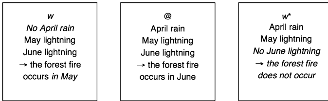
Fig. 4 The three worlds that are relevant for evaluating security-dependence in Delayed forest fire ; I have used italics to emphasise differences from the actual world @. Note that @ is here placed in the middle; this is intended to reflect the fact that w differs from @ in one way, while w^* differs from @ in another way
