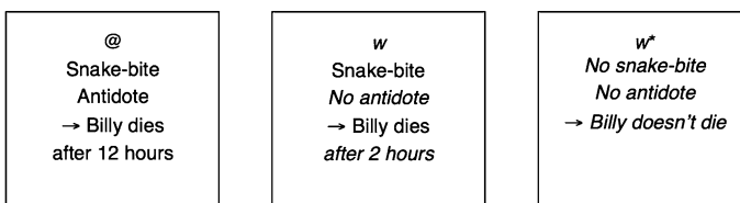
Fig. 6 The three worlds that are relevant for evaluating security-dependence in Fatal antidote ; I have used italics to emphasise differences from the actual world @. Note that I have put the actual world, @, on the far left, since this order of the worlds best reflects the comparative similarity between them
