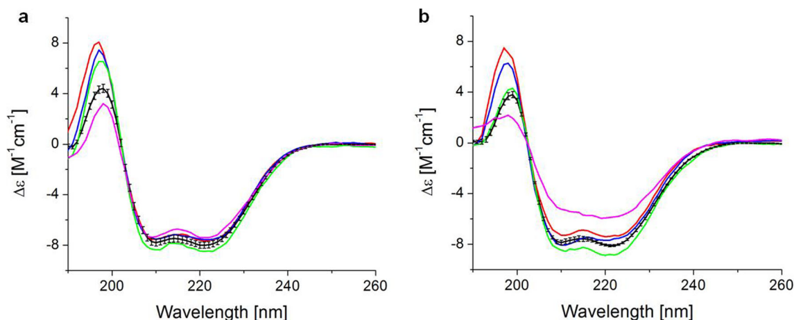
Fig. 2 Circular dichroism spectra of filgrastim products at (a) 25 and (b) 55°C. Average curve represents the spectra of the expired bathes of Neupogen (black line), Neupogen batch 1056681 (red line), Tevagrastim (blue line), Biocilin (green line) and PDgrastim (pink line).
