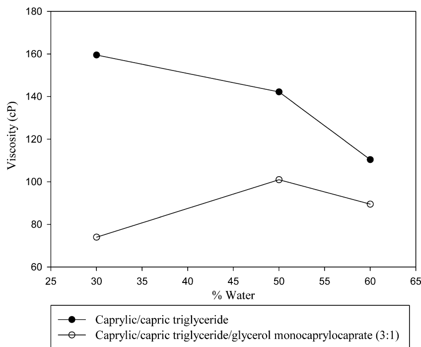
Fig. 6 Comparison of viscosities (25°C) vs. percent water for caprylate/ capric triglyceride (Captex 355) and the mixture of caprylate/ capric triglyceride and glycerol monocaprylocaprte at 2:8 lipid to surfactant (Cremophor EL) ratio.
