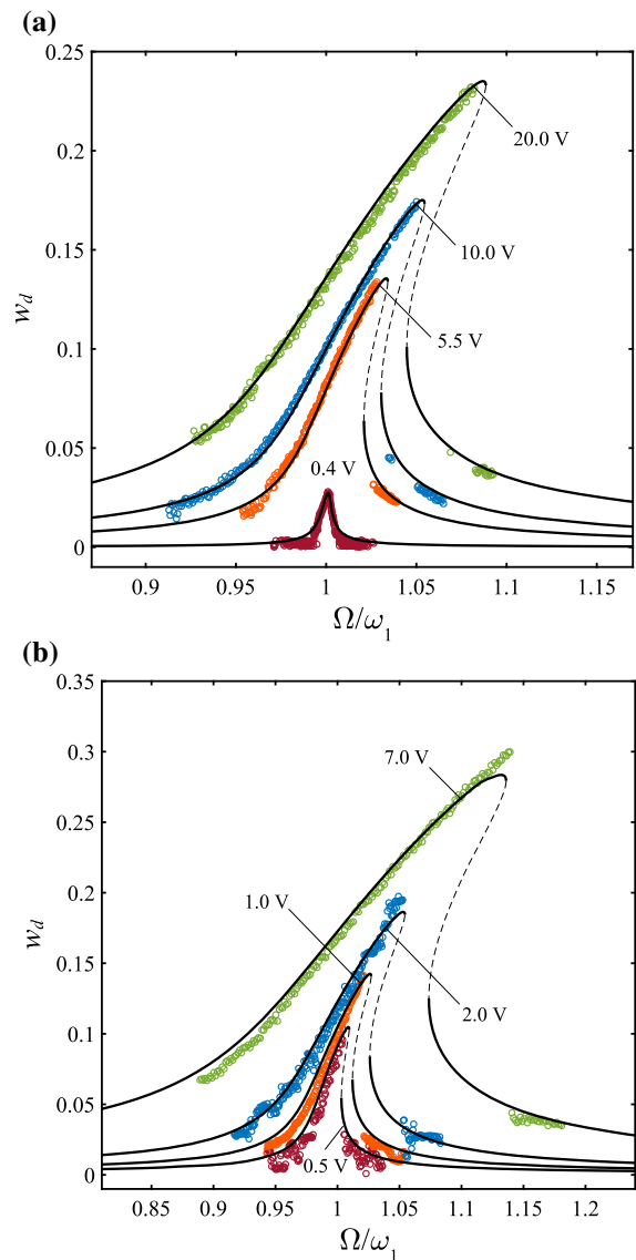
Fig. 7 Frequency responses of the MEMS resonator at a V_{DC} = 5\text{ V} and b V_{DC} = 30\text{ V} , and various AC voltages (denoted on the curves). Circles: experimental data; lines: theoretical predictions using the general quadratic-cubic damping model with the three damping coefficients calibrated based on the experimental data for V_{AC} = 0.4, 5.5, and 10\text{ V} (sub-figure (a))
