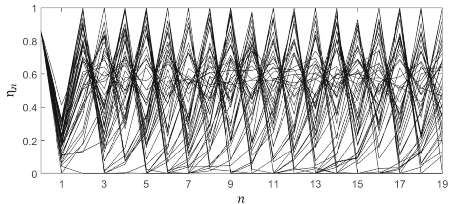
Fig. 8 Crossovers in the time series of \mathcal{S}(x_n) with x_0 = 0.8633 for \nu = 0.3 and SNR = 20 dB
