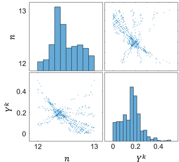
Fig. 16 Crossover solutions in the noisy trajectory of \mathcal{B}(x_n) between iterations 12 and 13 with the histogram showing the concentration of Y^k solutions around the fixed point
