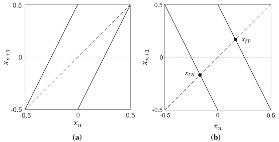
Fig. 14 Bernoulli map with a \beta = 1 and b intersection with diagonal appearing for -\mathcal{B}(x_n) with \beta = 1
