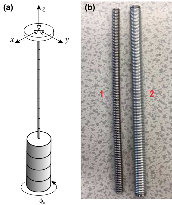
Fig. 8 a Setup of the apparatus used to determine the damping and the torsion stiffness of the flexible shafts (adopted from [2]) and b photograph of the two flexible shafts
