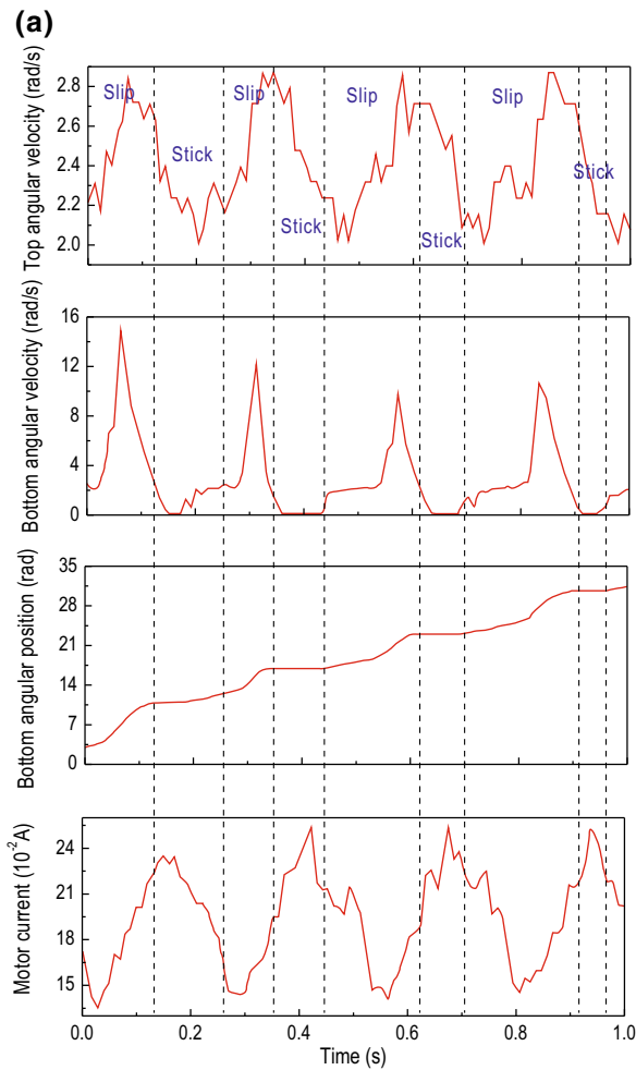
Fig. 15 Experimental results of Test 6. The time histories of top angular velocity, bottom angular velocity, bottom angular position, and motor current are presented for \kappa = 2.46 \times 10^{-2} \text{ m}^4 ,
