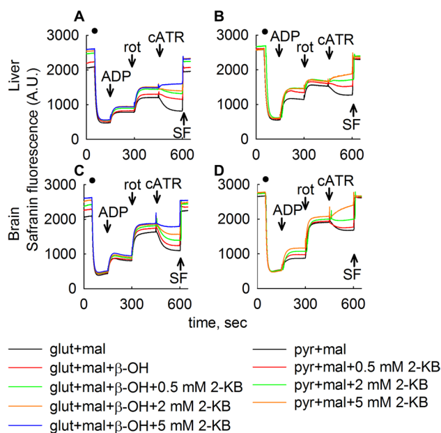
Fig. 4 2-KB abolishes mSLP. Reconstructed time courses of safranin O signal in isolated mouse liver (a, b), or brain (c, d) mitochondria. Mitochondria were added where indicated by the closed circles. ADP (2 mM) was added where indicated. The effect of cATR (2 \mu M) on \Delta\Psi_m treated with rotenone (rot, 1 \mu M) in the absence or dose-dependent presence of 2-KB as indicated in the legends is shown. Control traces are shown in black. At the end of each experiment 250 nM SF 6847 was added to achieve complete depolarization (an increase in safranin O fluorescence signal implies depolarization). Wherever single graphs are presented, they are representative of at least four independent experiments
