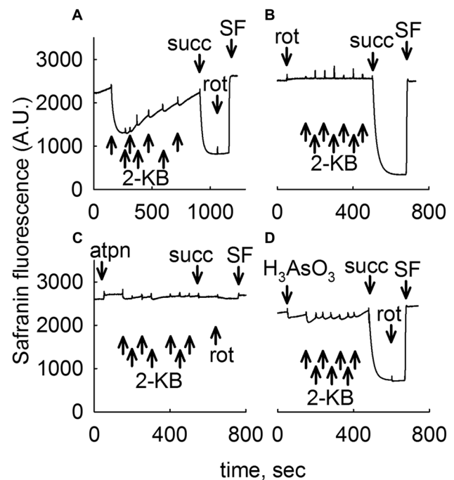
Fig. 2 2-KB as a metabolic fuel in mouse liver mitochondria. Reconstructed time courses of safranin O signal in isolated mouse liver mitochondria. The effect of 2-KB pulses (indicated by arrows signifying 0.5 mM each, thus a total of 3.5 mM 2-KB added) is shown. Whenever indicated, succinate (5 mM) or rotenone (1 \mu M) or atpenin (atpn 1 \mu M), or arsenite ( H_3AsO_3 , 1 mM) was added. At the end of each experiment 250 nM SF 6847 was added to achieve complete depolarization (an increase in safranin O fluorescence signal implies depolarization). Wherever single graphs are presented, they are representative of at least 4 independent experiments
