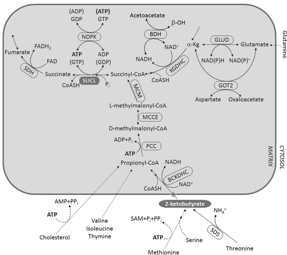
Fig. 1 Catabolism of metabolites towards succinyl-CoA. BCKDHC: branched-chain keto-acid dehydrogenase; BDH: \beta -hydroxybutyrate dehydrogenase; GLUD: glutamate dehydrogenase; GOT2: aspartate aminotransferase; KGDHC: ketoglutarate dehydrogenase complex; MCM: methylmalonyl mutase; MCEE: methylmalonyl racemase; NDPK: nucleoside diphosphokinase; PCC: propionyl-CoA carboxylase; SAM: S-adenosylmethionine; SDH: succinate dehydrogenase; SDS: L-serine dehydratase/L-threonine deaminase; SUCL: succinate-coA ligase. Dashed arrows imply multiple steps which may occur inside or outside the mitochondrial matrix. Entrance of 2-KB into the matrix likely occurs through the mitochondrial pyruvate carrier (depicted by a grey semi-transparent cylinder)
