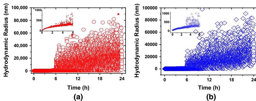
Fig. 2 Aggregation characteristics of gold nanoparticles in physiological condition a 30 nm samples, b 60 nm samples
