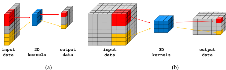
Fig. 3 a 2D convolution operation; b 3D convolution operation
