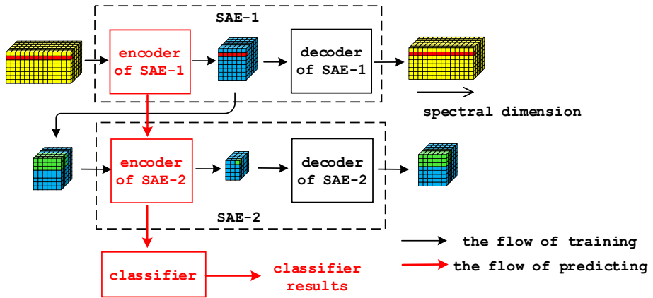
Fig. 4 Framework of TMC-SAE
