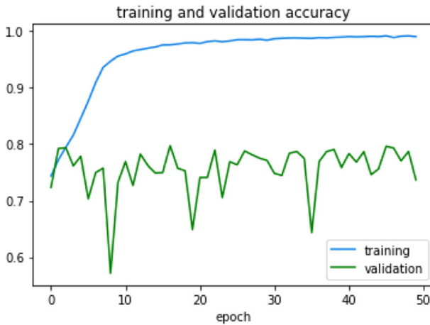
Fig. 38 Training and validation accuracy of InceptionV3
