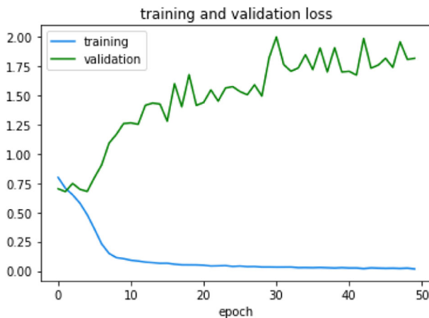
Fig. 21 Training and Validation loss of ResNet152
