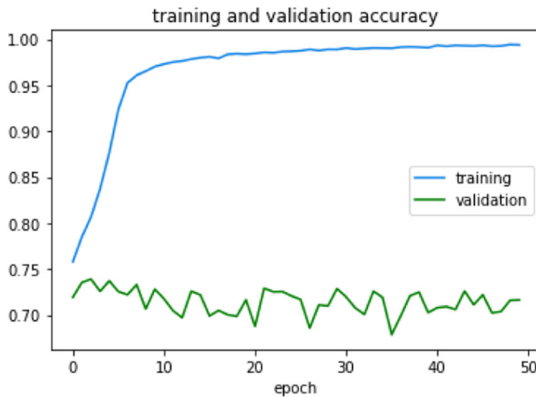
Fig. 18 Training and Validation accuracy of ResNet50
