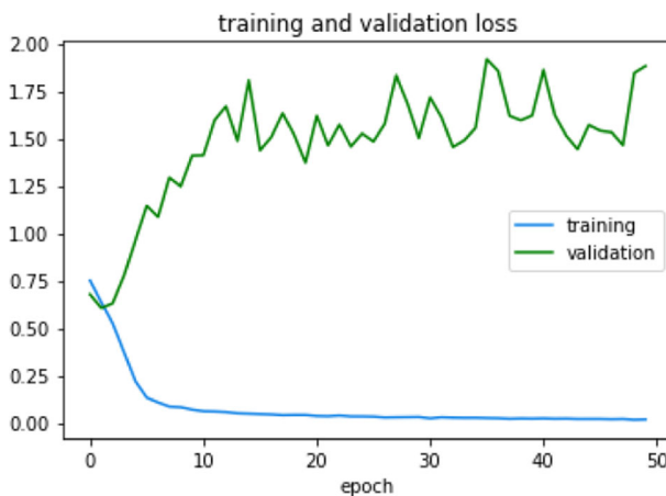
Fig. 35 Training and validation loss of Xception
