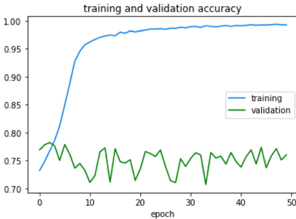
Fig. 24 Training and Validation accuracy of ResNet152V2
