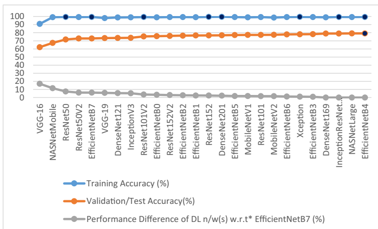
Fig. 65 Performance accuracy of 26 DL models w.r.t EfficientNetB7
