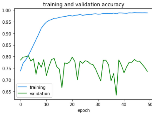
Fig. 26 Training and validation accuracy of DenseNet121
