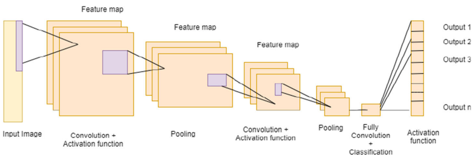
Fig. 1 Block diagram of CNN
