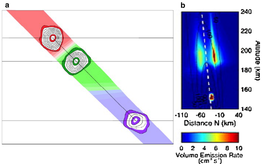
Fig. 2 a Arecibo observations April 20, 1988, 15 s integrations, in projection of HF electron excited optical emission contours (derived as in Fig. 1) for 630.0 nm (in red), 557.7 nm (in green) and 777.4 nm (in violet), horizontally aligned in the magnetic meridian plane, then moved vertically along the magnetic field line over Arecibo Observatory. The vertical scale is about half a neutral oxygen scale height (tens of km). b HAARP observations (Pedersen et al. 2010) of 557.7 nm images for 210 s combined by a tomographic algorithm, giving a cross-cut of the optical volume emission rate in the magnetic meridian plane (140–240 km altitude vs. –110 to +40 km North of overhaed the HF heater). The HAARP magnetic field line and contours of nominal transmitter power in percent relative to peak power at 230 km altitude are superimposed on the tomographic map
