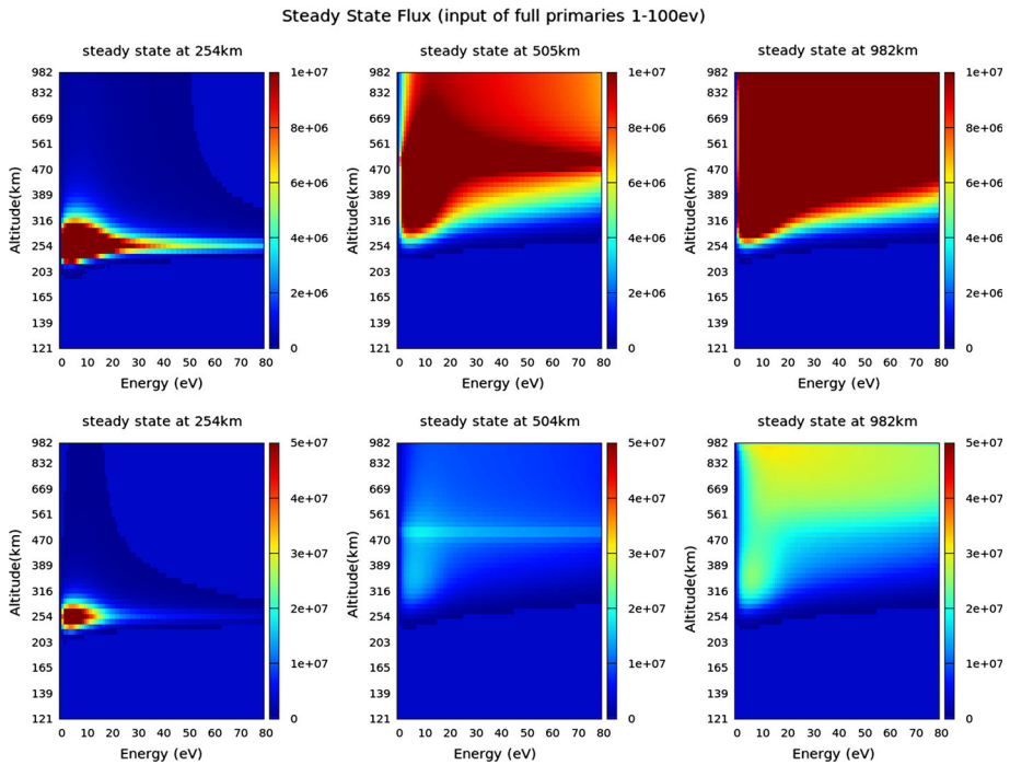
Fig. 4 Shows the results for a single thin altitude source slab of HF accelerated electrons at three altitudes, one at which the thermosphere is: very optically thin (982 km) far right hand side, intermediate (505 m) center, one at a depth at which the thermosphere is optically thick (254 km) left hand side of figure, and one intermediate (505 km) in the central column of the figure. The only difference between the top and bottom row is the flux scale, to visualize a dynamic range of a factor of 50 in suprathermal flux. This shows penetration depth of composite electron flux including all primary and secondary electrons
