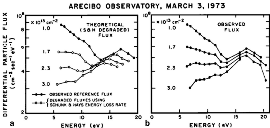
Fig. 6 a Differential particle fluxes ( \text{electrons cm}^{-2} \text{s}^{-1} \text{eV}^{-1} ) obtained by degrading the experimental spectrum shown in and Abreu and Carlson (1977) Figures 5a and 8b at 1.0 \times 10^{13} \text{cm}^{-2} using the Schunk and Hays (1971) energy loss expression; b the observed differential particle fluxes for matched conditions
