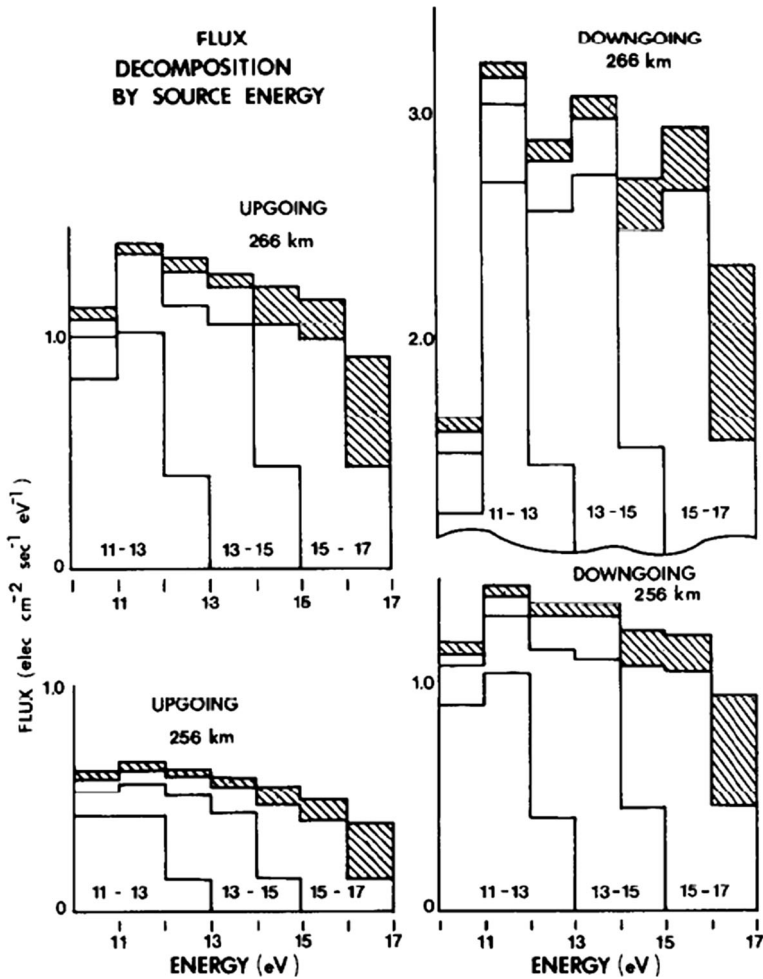
Fig. 3 Relative fluxes of up-going and down-going suprathermal electrons at several altitudes in the observation region were derived from a uniform production rate from zero to 20 eV electrons, all originating at 275 km. This figure shows their decomposition by energy of the up-going and down-going suprathermal electron fluxes (electrons \text{cm}^{-2} \text{s}^{-1} \text{eV}^{-1} ) at 256 and 266 km. The calculations partition electrons into 2 eV segments of the spectrum at 275 km, and were traced to other energy ranges at lower or higher altitudes. The right-hand figure shows the downward flux at the two altitudes. The left-hand figure shows the upward flux obtained from electrons backscattered at the indicated and lower altitudes (Carlson et al. 1982)
