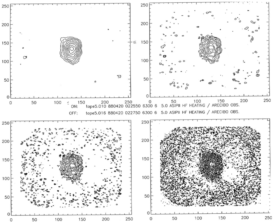
Fig. 1 Original data Arecibo April 20, 1988, for 630.0 nm emission and surrounding background, in single frame image, with no data processing beyond increasing degrees of smoothing of adjacent pixels, to reduce noise fluctuations in image. Clear contours stand out well against background with no further subtraction
