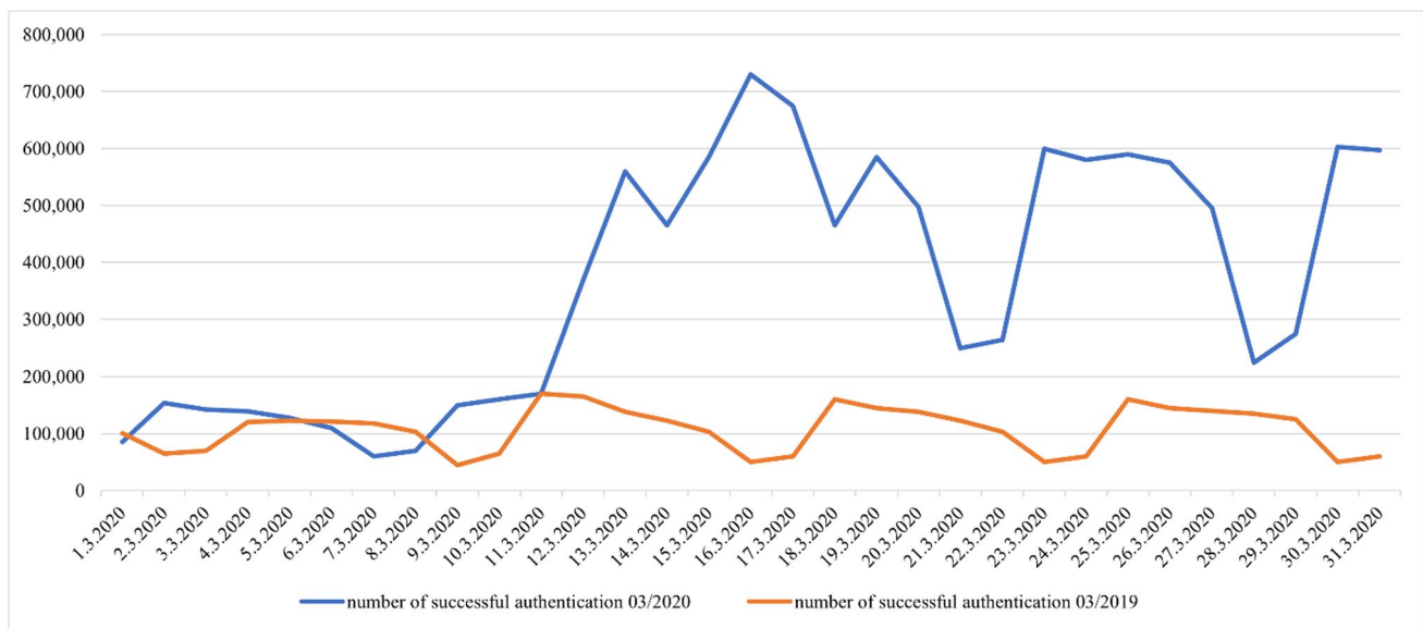
Fig 5 Number of successful authentications of March 2019 and 2020 comparison
