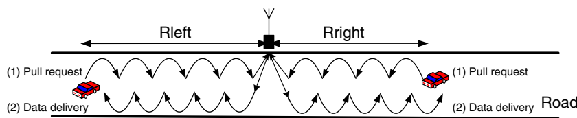
Fig. 2 Coverage of pull. The requesting car (either at left or right of the infostation) first sends out a pull request towards its nearest infostation, forwarded by vehicles in the middle. The infostation
