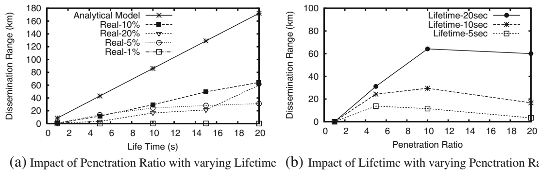
Fig. 11 The pull scheme (real trace). Impact of penetration ratio. Dissemination range increases as penetration ratio increases from 1–10%. Further increase in penetration ratio leads to in-
