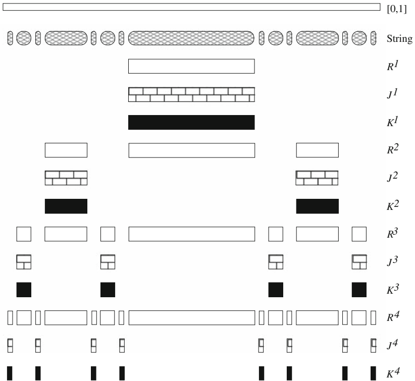
Figure 5. Construction of the multifractal zeta function \zeta_{\mathcal{N}}^{\mu}(\infty, s) as in the proof of Theorem 4.2.
