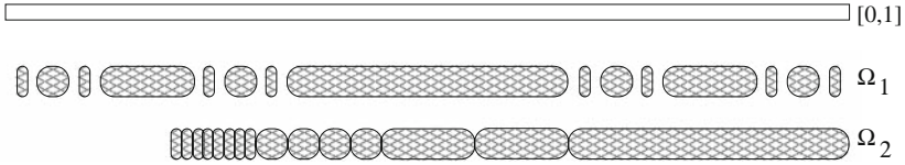
Figure 2. The first four distinct lengths, with multiplicities, of the Cantor String \Omega_1 and the fractal string \Omega_2 .
