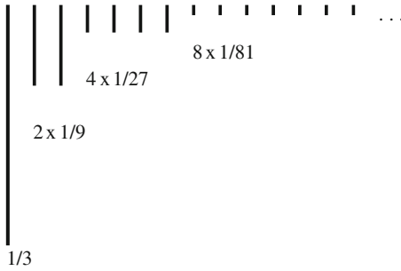
Figure 1. The lengths of the Cantor String.
