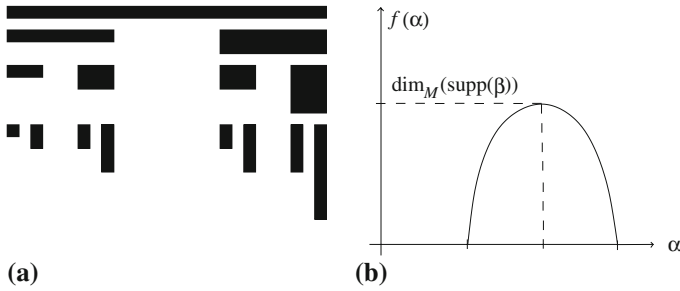
Figure 3. a Construction of the binomial measure \beta . b The multifractal spectrum f(\alpha) of the measure \beta .
