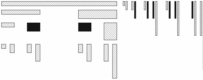
Figure 9. The first stages in the construction of the partition zeta function \zeta_{\mathfrak{P}}^{\beta}(\alpha(1, 2), s) whose regularity \alpha = \alpha(1, 2) yields the maximum value of the multifractal spectrum f(\alpha) of the binomial measure \beta . The solid black bars contribute their lengths to the series formula of the partition zeta function.
