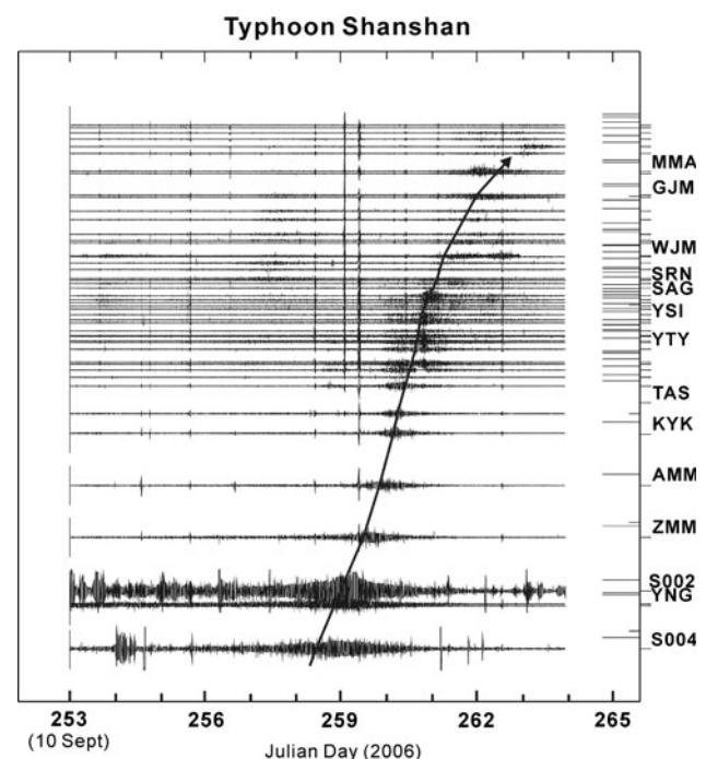
Fig. 2 Stack plot showing how Typhoon Shanshan was recorded. The solid line with an arrow marks the time when the typhoon is closest to the station. This figure suggests the major source region is moving with and trailing behind the typhoon. This figure is reproduced from Chi et al. (2010, Fig. 2)
