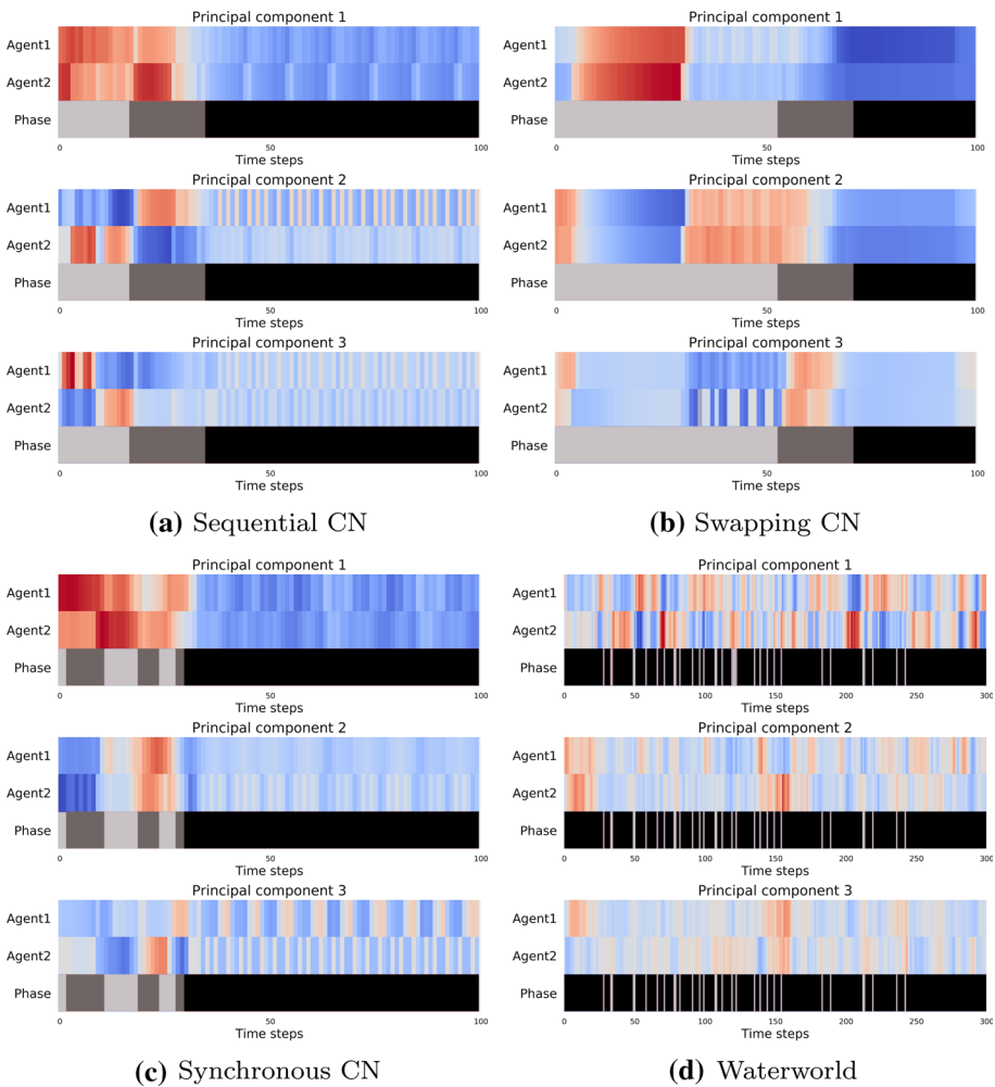
Fig. 3 Visualisation of communication strategies learned by the agents in four different environments: the three principal components provide orthogonal descriptors of the memory content written by the agents and are being plotted as a function of time. Within each component, the highest values are in red, and the lowest values are in blue. The bar at the bottom of each figure indicates which phase (or sub-task) was being executed within an episode; see Sect. 4.4 for further details. The memory usage patterns learned by the agents are correlated with the underlying phases and the memory is no longer utilised once a task is about to be completed (Color figure online)
