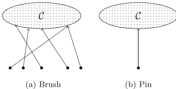
Fig. 5 An example of a brush and of a pin, where the top ellipses illustrate the final clusters and an arrow relates the state it started from to every element in the cluster
