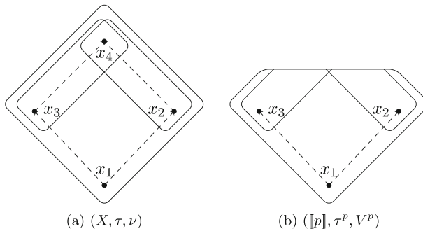
Fig. 4 Update of (X, \tau, \nu) by p
