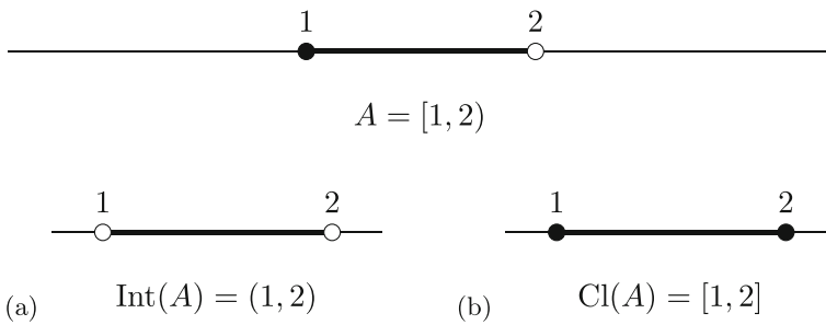
Fig. 1 The natural topology on \mathbb{R}
