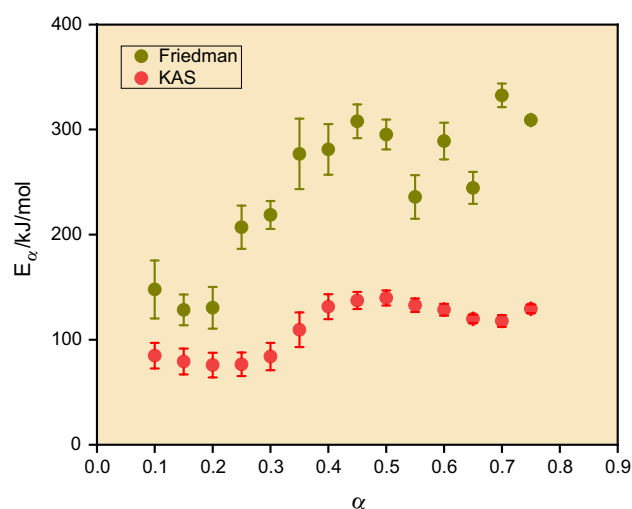
Fig. 4 Dependence of the activation energy E_\alpha as function of the extent of conversion ( \alpha ) for the thermal decomposition of GPD in N_2 between 180 and 750 \text{ }^\circ\text{C} using the FR and KAS methods
