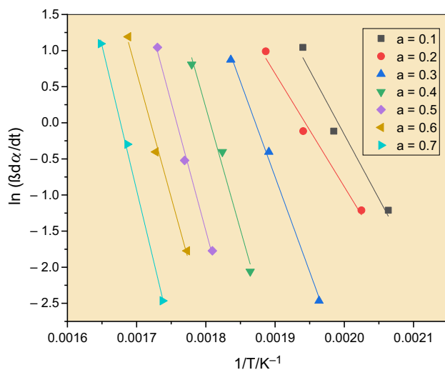
Fig. 3 Arrhenius plots for the thermal decomposition of GPD in N_2 between 180 and 750 \text{ }^\circ\text{C} using the FR method
