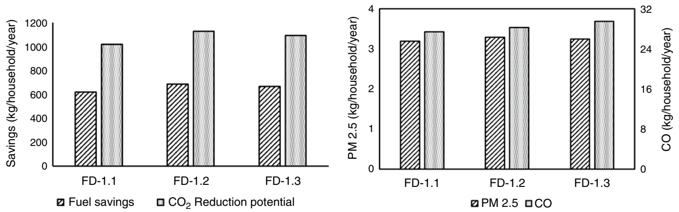
Fig. 12 Annual fuel savings and emission reduction potential of CO, PM 2.5 and CO 2 from forced draft cookstove models
