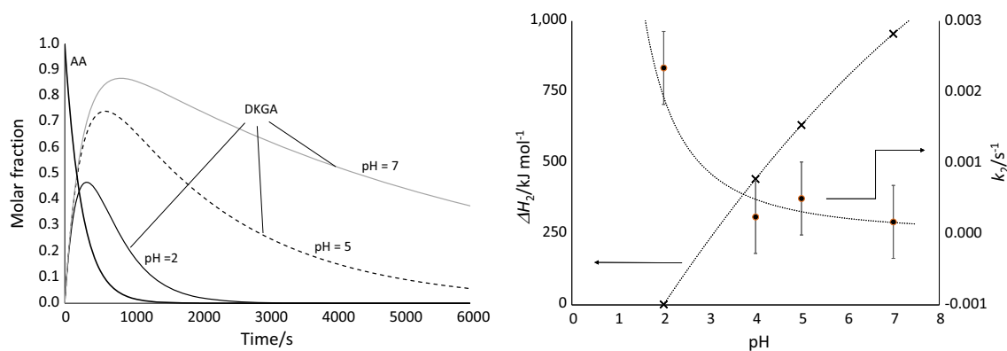
Fig. 14 Trends of the molar ratios of AA and DKGA at various pH. Kinetic constant and enthalpy drop of the second step of the two consecutive step model
