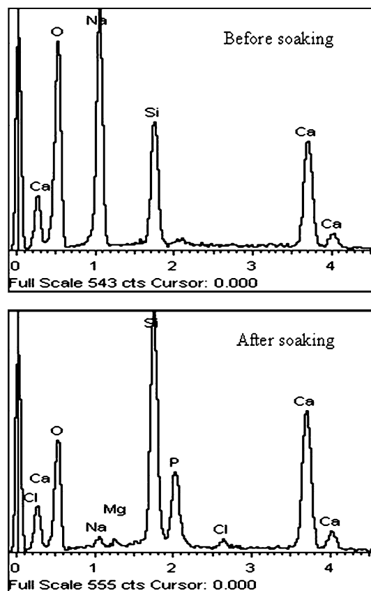
Fig. 4 EDS spectra of \text{Na}_2\text{CaSiO}_4 disks before and after soaking in SBF for 7 days
