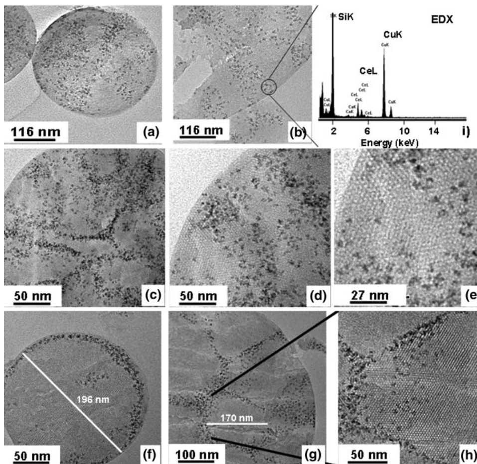
Fig. 3 Microtomed TEM images of mesostructured silica embedding: (a, b) non-modified, (c–e) phenyl-modified and (f–h) amino-modified cerium oxide nanoparticles. (i) EDX spectrum of ceria-containing silica obtained during TEM measurements
