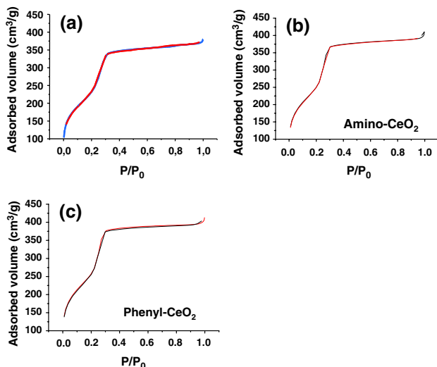
Fig. 2 N 2 adsorption/desorption isotherms of spray-dried mesoporous silica particles embedding (a) non-functionalized and (b) amino- and (c) phenyl-functionalized cerium oxide nanoparticles
