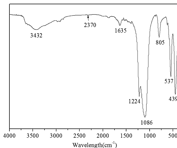
Fig. 1 FT-IR spectrum of NKF-5 zeolite
