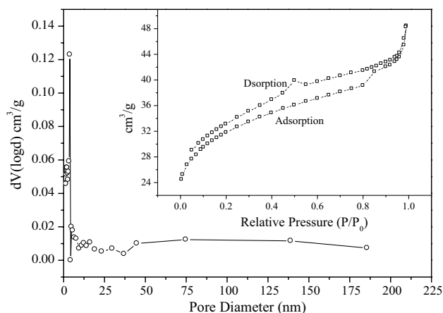
Fig. 3 N 2 adsorption–desorption isotherms (insert) and corresponding BJH pore-size distribution curve of Na-rectorite sample
