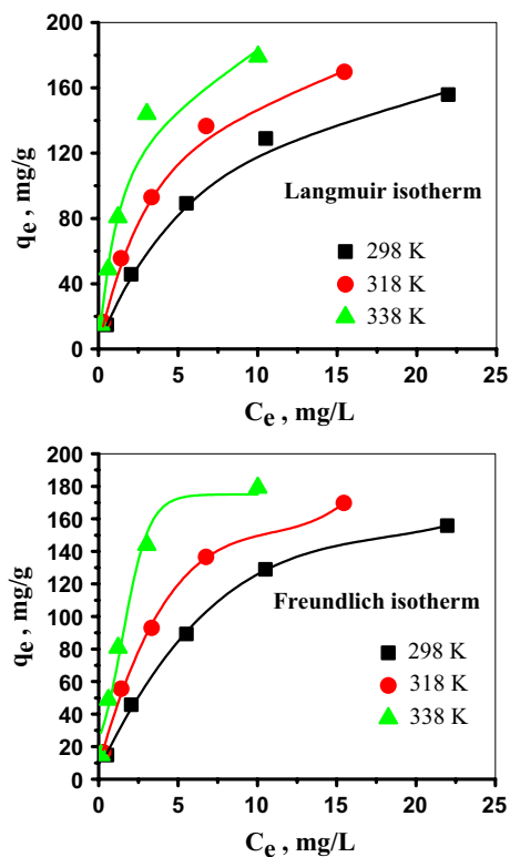
Fig. 8 Langmuir and Freundlich isotherms for 60 Co radionuclide sorption onto prepared CS–CuO with humic acid
