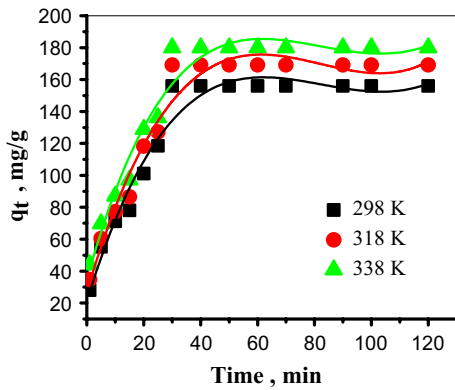
Fig. 10 Pseudo-second-order kinetic model for ^{60}\text{Co} radionuclide sorption onto prepared CS–CuO with humic acid
