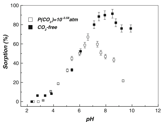
Fig. 14 Effect of CO 2 on U(VI) sorption on DCS as a function of pH values. C[\text{UO}_2^{2+}]_{\text{initial}} = 2.86 \times 10^{-5} mol/L, I = 0.05 mol/L NaClO 4 , m/V = 0.4 g/L, T = 25 \pm 1 °C. ■: CO 2 -free, □: P(\text{CO}_2) = 10^{-3.58} atm
