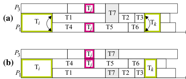
Fig. 6 Transforming a non-contiguous schedule on m = 3 to a contiguous schedule
