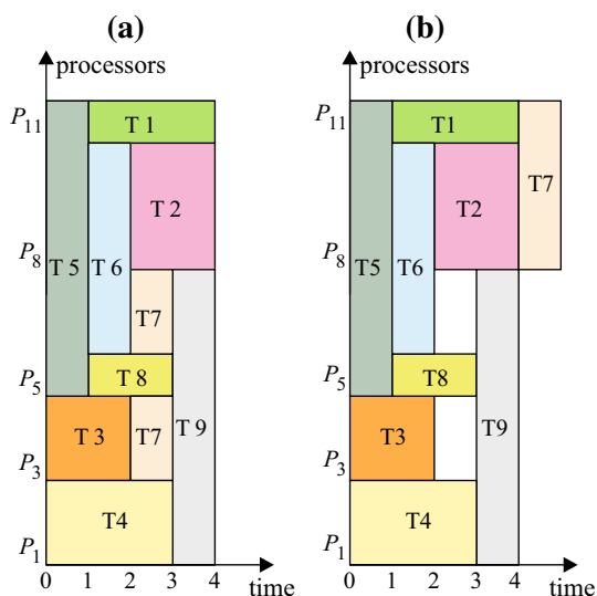
Fig. 5 C /nc-difference with the shortest possible C_{\max}^{nc} . a Optimum non-contiguous schedule, b optimum contiguous schedule
