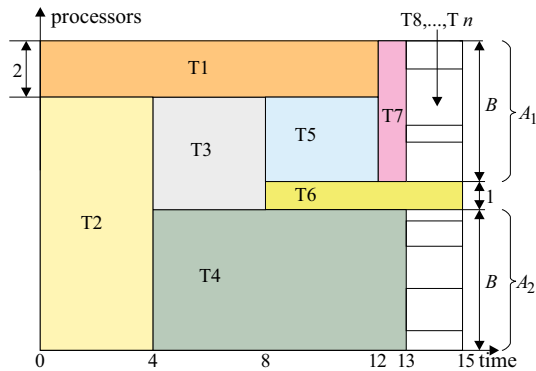
Fig. 7 Schedule for the proof of Theorem 5
