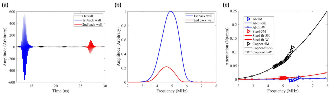
Fig. 4 Experimental results obtained from a 5 MHz shear wave PZT plate; a , b the time domain back-wall signals and their spectra from the copper specimen and c the comparison of measured shear wave attenuation on different materials
