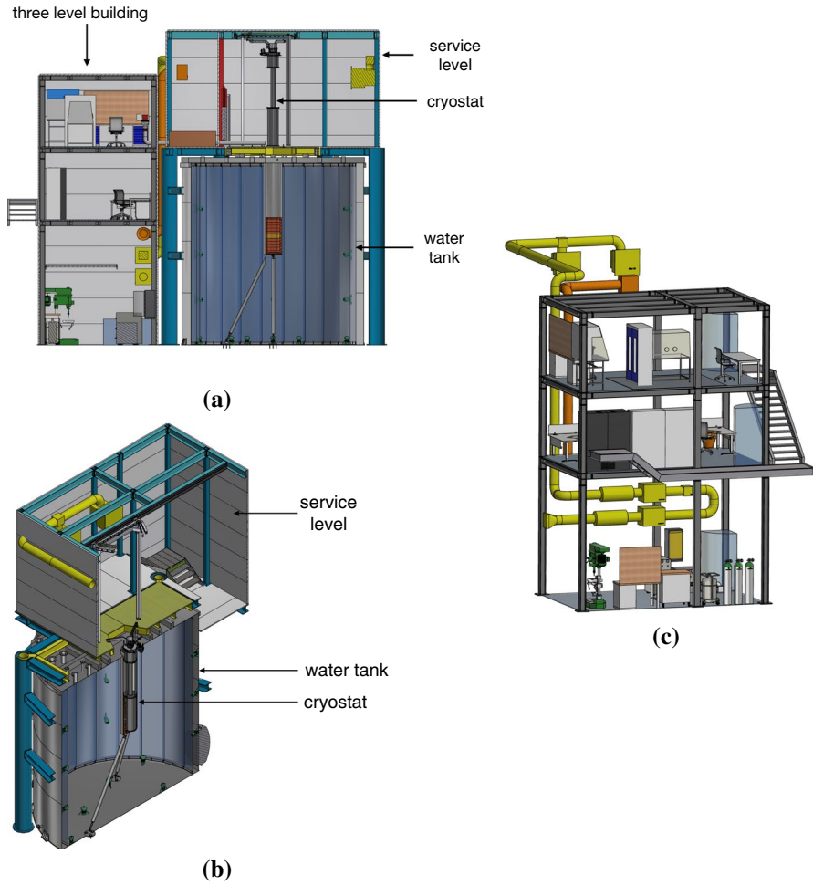
Fig. 2 The scheme shows a preliminary 3D section of the COSINUS experimental set-up as located in hall B of LNGS. The cryostat hosting the COSINUS detectors is inserted in the dry well of a 7 × 7-m water tank. Panel a : the cryostat lifted up from the dry well to the servicing level. The servicing level equipped with a clean room allows for detector mounting. The three-level building close to the water tank will host the DAQ and the electronics, the cryostat-related infrastructure and a working area. Panel b : sectional view of the cryostat inserted in the dry well of the water tank and, on top of the water tank, the service level. Panel c : 3D view of the three-level control building (color figure online)
