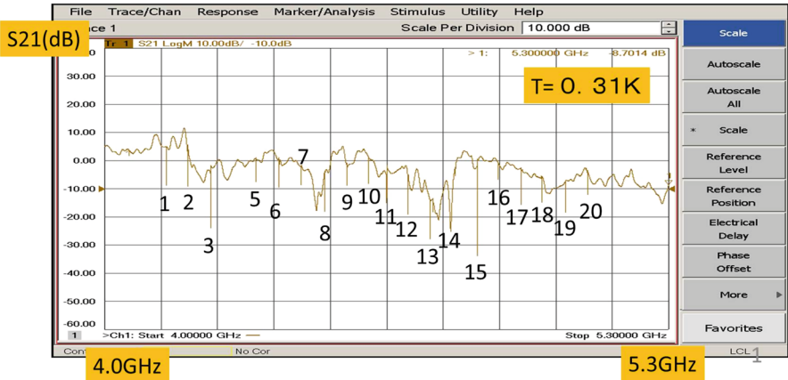
Fig. 2 Resonant peaks measured by a vector network analyzer. The numbers correspond to the resonators of the top figure in Fig. 1. (Color figure online)
